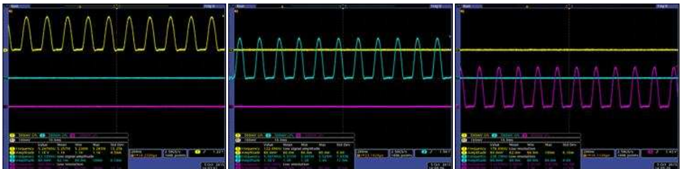
Figure 7. Proximity Sensor Waveform (Yellow), Cap Touch Button 1/2 Waveforms (Green and Magenta)
