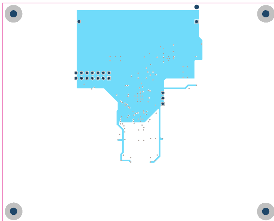
Figure 13. Midlayer 2 (GND Plane)
