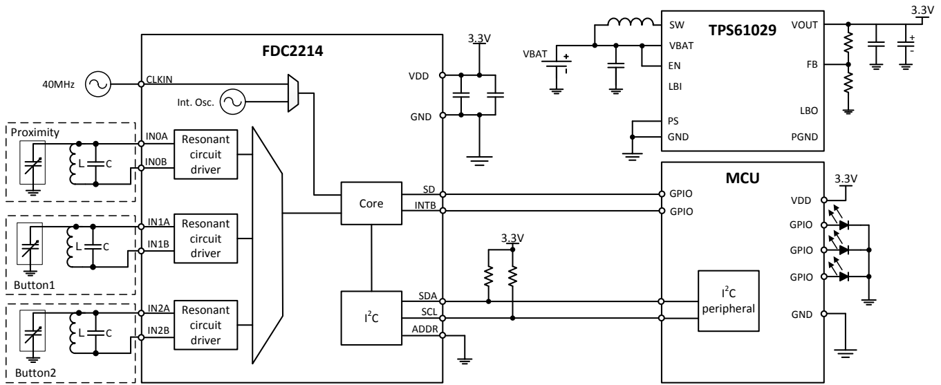
Figure 2. System Level Block Diagram
