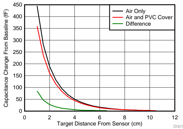
Figure 5. Comparison of Capacitance vs Target Position for Covered and Non-covered Sensors
