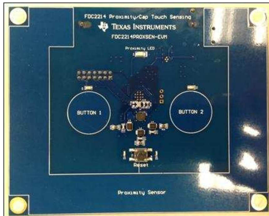
Figure 1. FDC2214 Proximity and Capacitor Touch Sensing EVM
