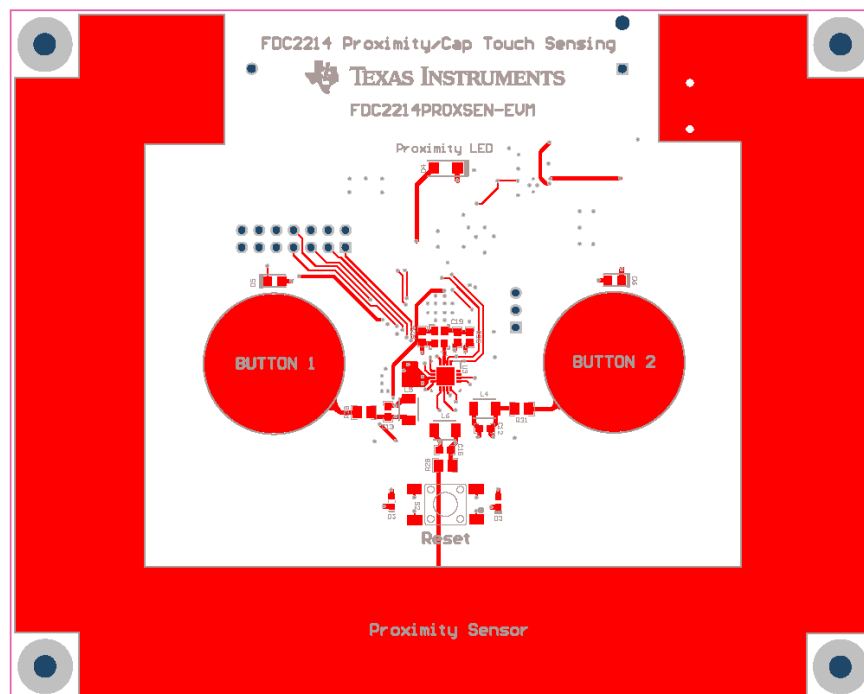
Figure 11. Top Layer
