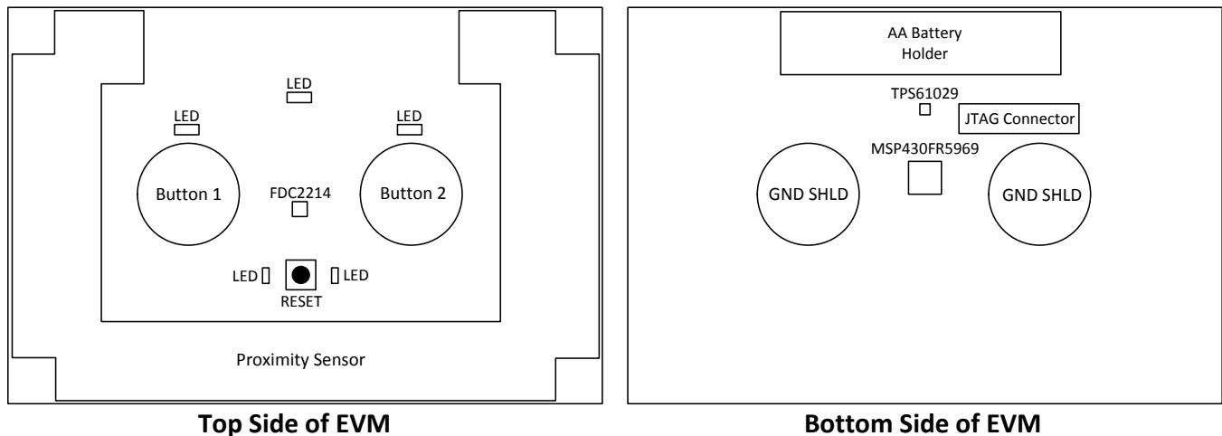
Figure 3. Component Layout Location of Board on Top Side and Bottom Side
