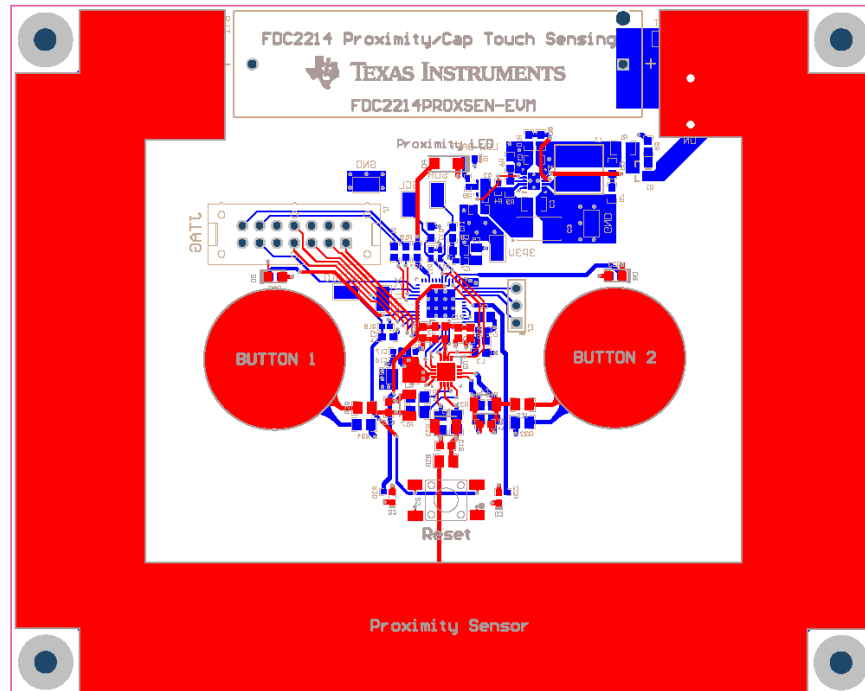
Figure 10. Composite Top and Bottom Layer Plot (Viewed From the Top)
