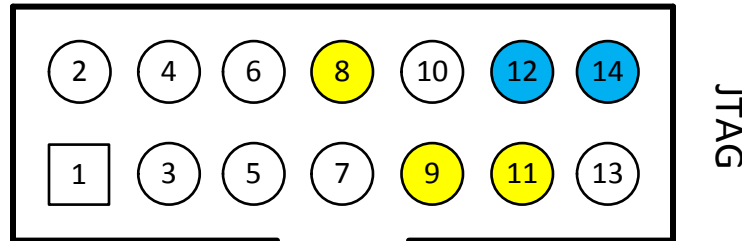
Figure 6. : JTAG Pin Out Diagram
