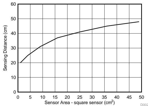
Figure 4. Sensor Size Area Versus Sensing Distance
