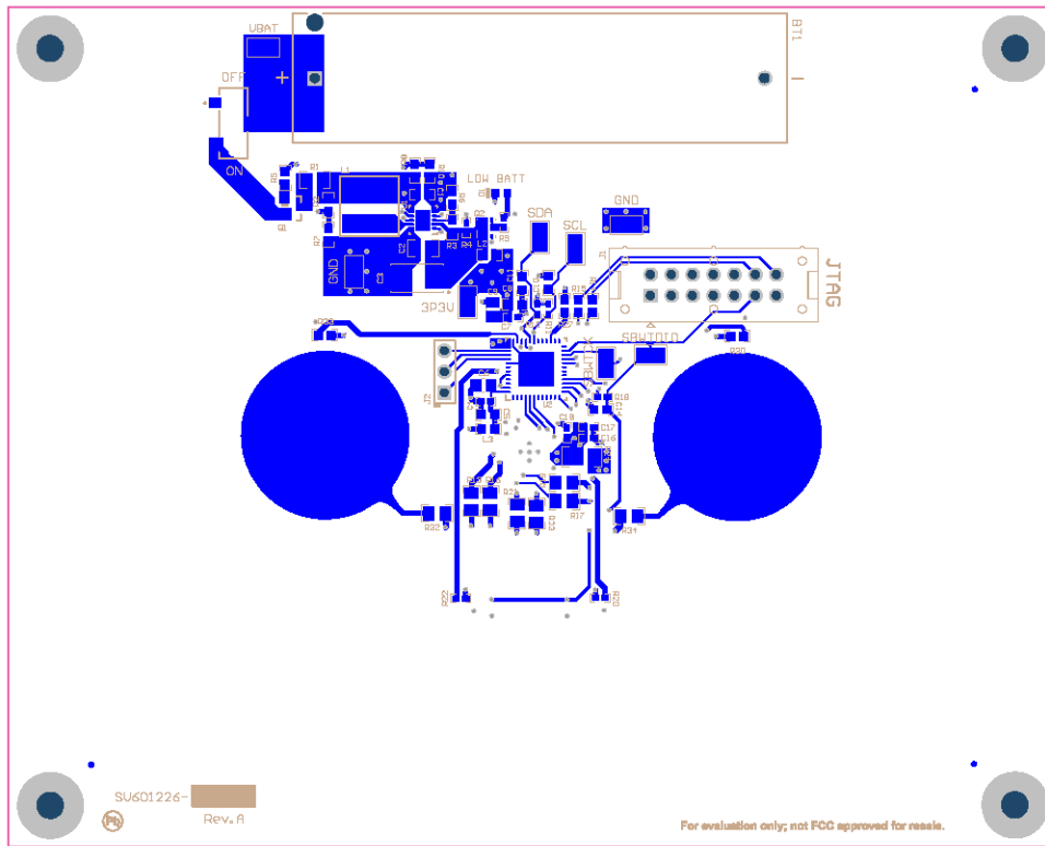
Figure 14. Bottom Layer
