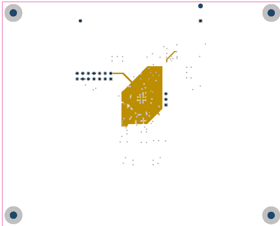
Figure 12. Midlayer 1 (Power Plane)
