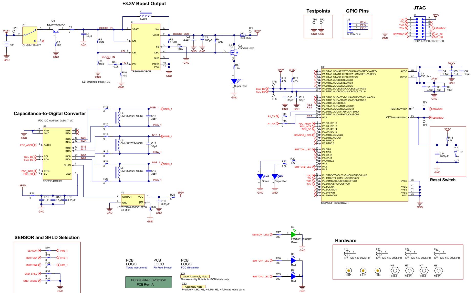
Figure 15. Schematic
