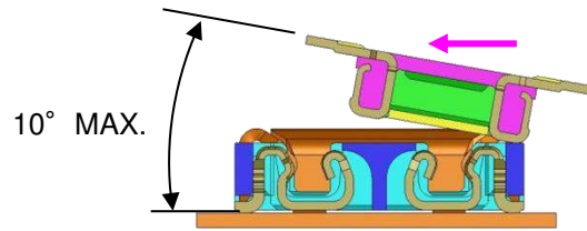
長手方向 "a" direction (lengthways)
