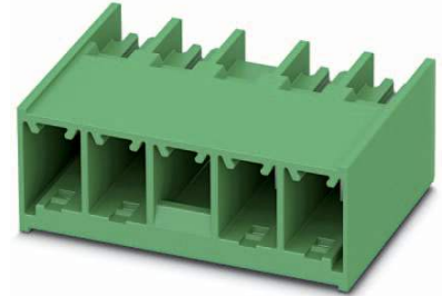
Figure shows a 4-pos. version with locking flange at position 3
