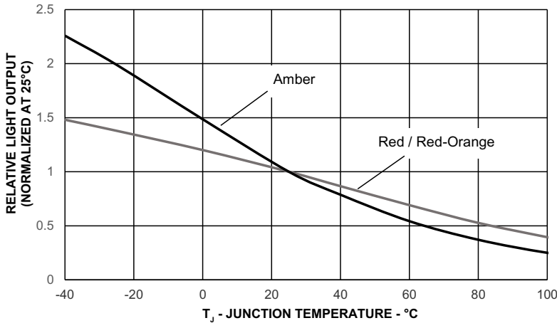
Figure 5: Relative Light Output vs. Junction Temperature
