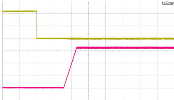
Fig. 9: Turn-on transient at full rated load current (resistive) with C_{out} 10 \mu F tantalum + 1 \mu F ceramic at V_{in} = 48 V, triggered via ON/OFF pin. Top trace: ON/OFF signal (2 V/div.). Bottom trace output voltage (1 V/div.). Time scale: 50 ms/div.
