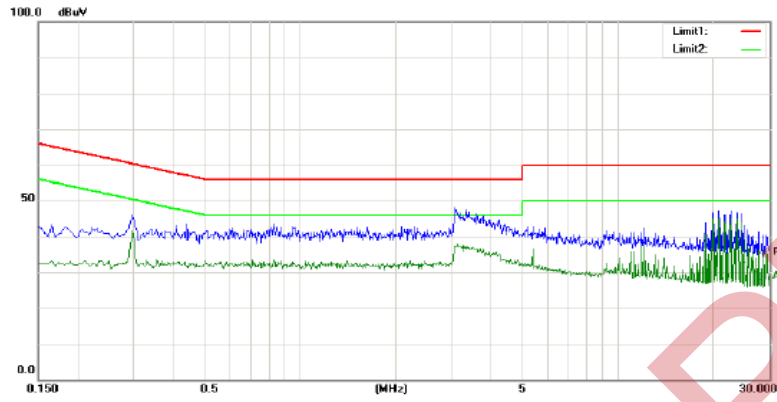
Fig. 19: Vin+ Peak Detector EMI waveform
