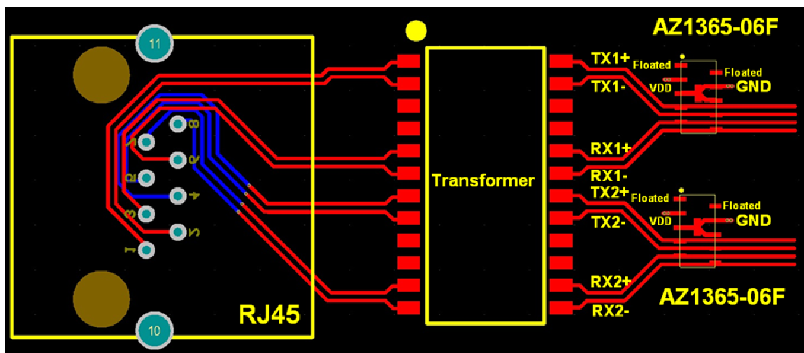
Fig. 4 The PCB layout of AZ1365-06F for an Ethernet port.
