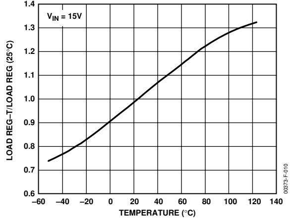
Figure 8. Normalized Load Regulation ( \Delta I_L = 10 \text{ mA} ) vs. Temperature
