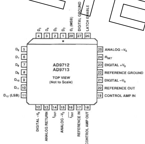
PLCC Pinout Designations
