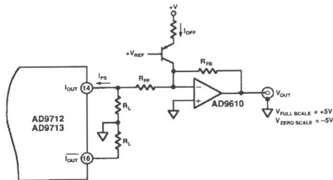
Figure 5. IV Conversion Using Current Feedback Amp
