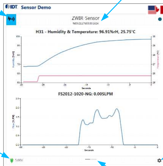
Figure 5. Overview of the Browser Display
