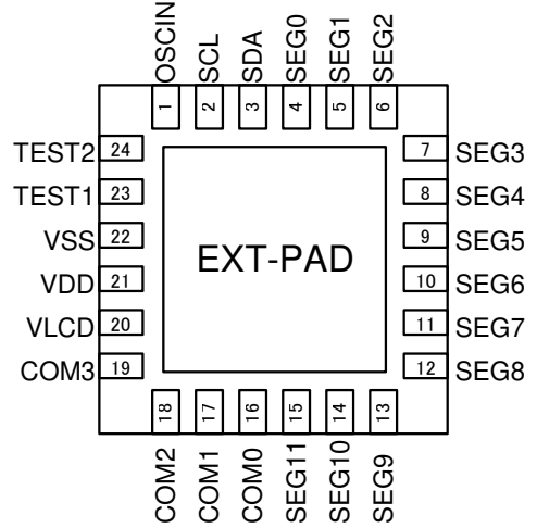
Figure 5. Pin Configuration (BOTTOM VIEW)
