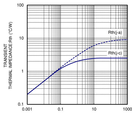
R_{th} \cdot t \text{ CHARACTERISTICS}
