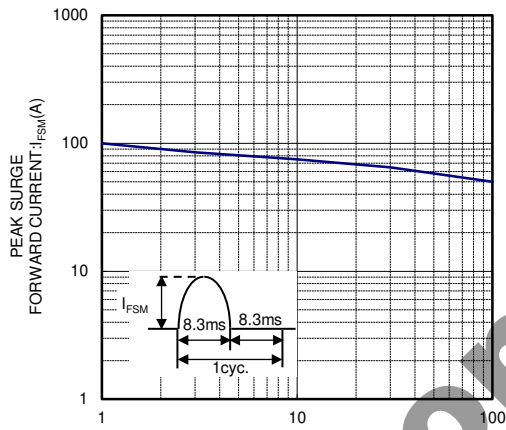
I_{FSM} \cdot \text{CYCLE CHARACTERISTICS}
