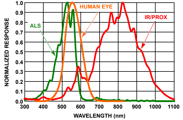
FIGURE 7. ISL29028 SENSITIVITY TO DIFFERENT WAVELENGTHS
