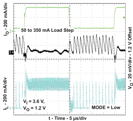
Figure 20. Load Transient Response in PFM/PWM Operation
