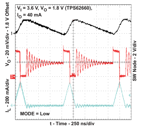
Figure 35. Power-Save Mode Operation
