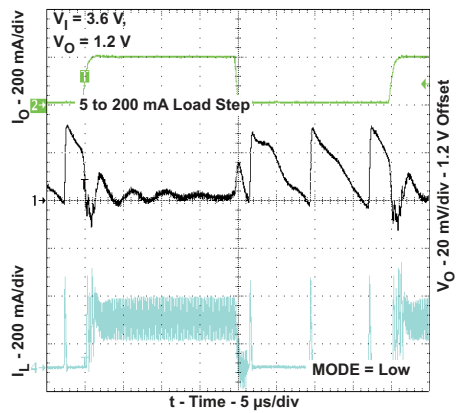
Figure 21. Load Transient Response in PFM/PWM Operation
