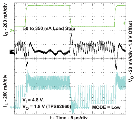
Figure 15. Load Transient Response in PFM/PWM Operation
