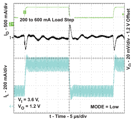
Figure 22. Load Transient Response in PFM/PWM Operation
