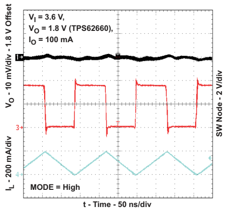
Figure 34. PWM Operation
