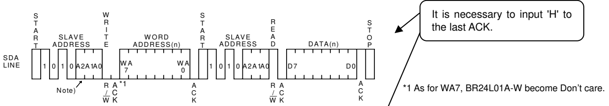
Figure 42. Random read cycle (BR24L01A/02/04/08/16-W)
