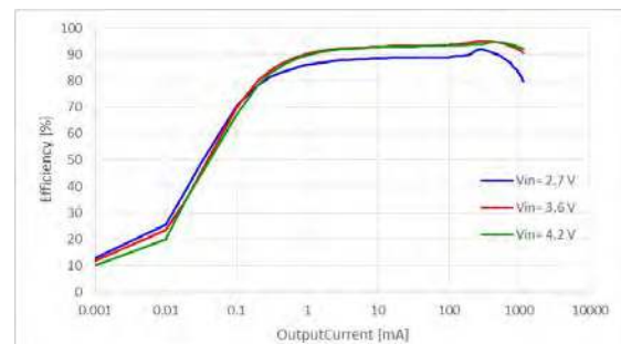
Efficiency Characteristics (RP602Z330x, MODE = H)
