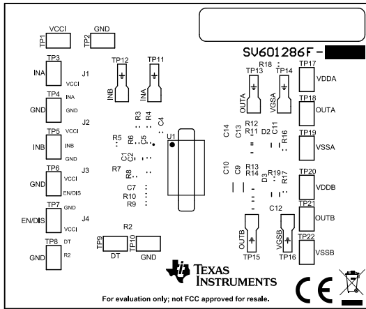
Figure 9-1. Top Overlay
