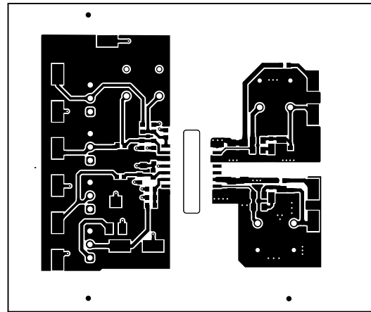
Figure 9-2. Top Layer
