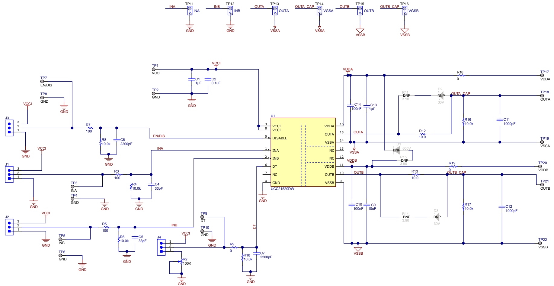
Figure 8-1. UCC21520EVM-286 Schematic
