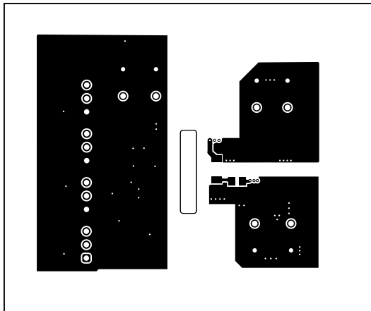
Figure 9-3. Bottom Layer
