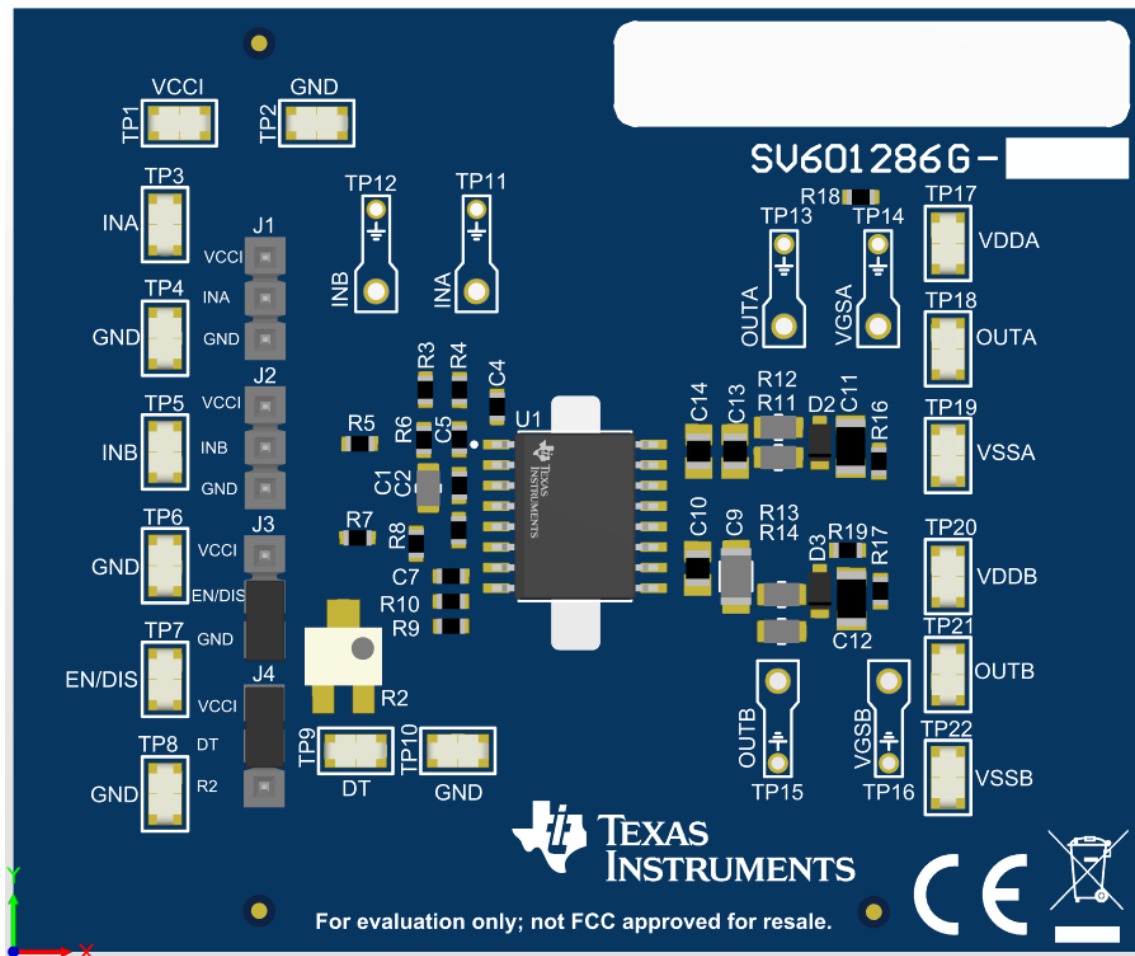
Figure 5-1. Jumpers Installation Position
