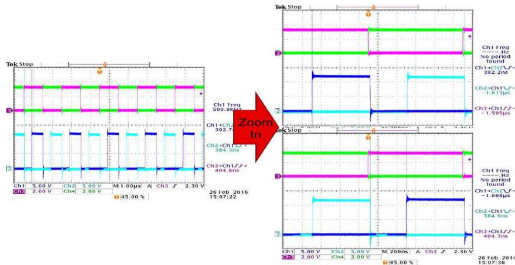
Figure 7-3. Test Waveforms if DT Connected to R_{DT} (Channel 3 and 4 is PWM Inputs, and Channel 1 and 2 is Driver Outputs)
