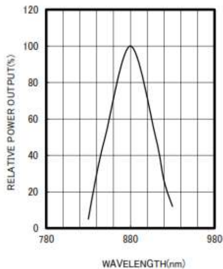
SPECTRAL OUTPUT
