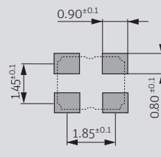
pad layout
