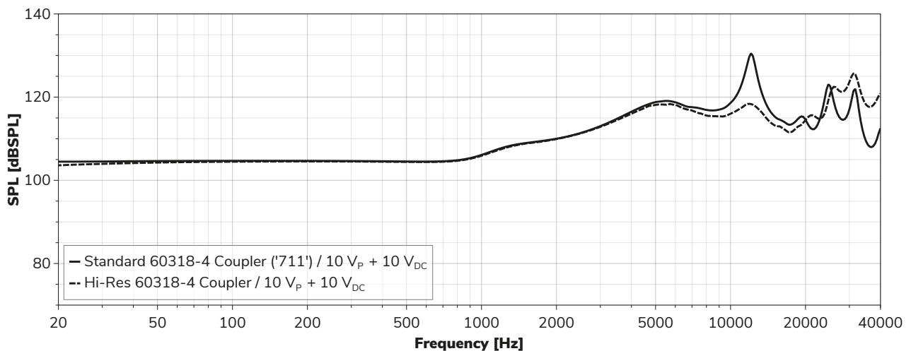
Figure 6: SPL at 7 V_{RMS} ( 10 V_p ) + 10 V_{DC} drive, measured with the standard 711-Coupler (IEC 60318-4) and with the Hi-Res Coupler from GRAS, the latter replicates the frequency response above 10 kHz more accurately
