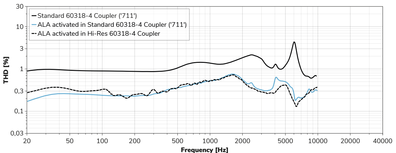
Figure 7: THD at 2.5 V_{RMS} ( 3.5 V_p ) drive (in logarithmic scale), measured with and without the ALA (see above) with the standard 711-Coupler (IEC 60318-4) and with the Hi-Res Coupler from GRAS. The latter replicates the frequency response above 10 kHz more accurately.
