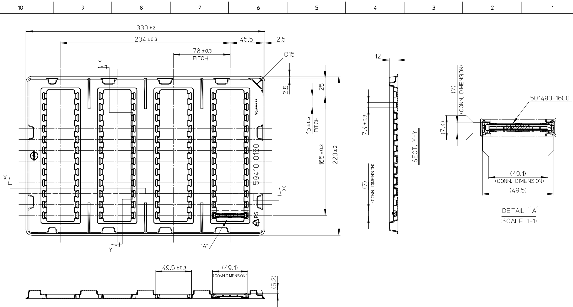
SECT. X-X
