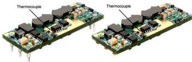
Fig. E: Locations of the thermocouples for thermal testing.
