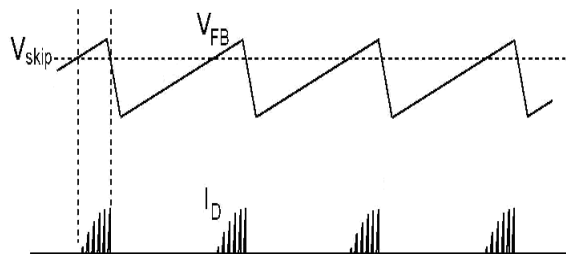
Figure 65. Soft-Skip™ operation.
