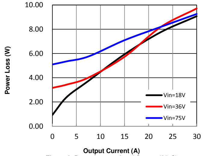
Figure 2. Power Loss vs. Load Current (25°C)
