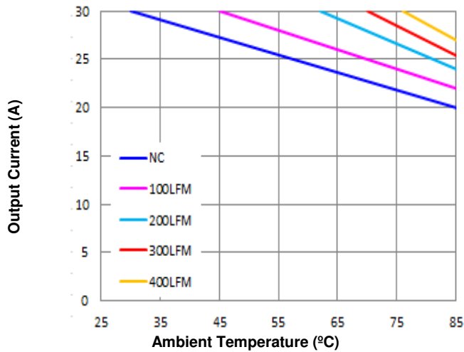
Figure 7. Current Derating Curve for Airflow Direction 3 (Ref. Fig. 8 for Airflow Direction; Vin = 36V, open frame)
