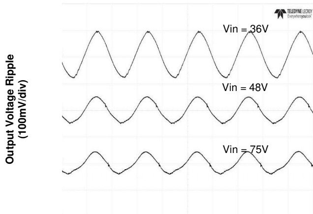
Figure 3. Output Voltage Ripple at Full Load
