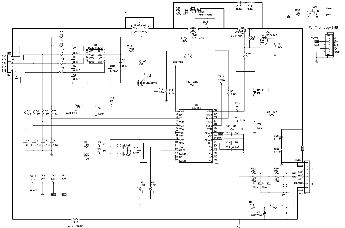
Figure 6. Application Schematic
