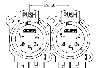
MINIMUM ASSEMBLY DISTANCE
