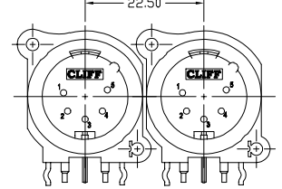
MINIMUM ASSEMBLY DISTANCE
