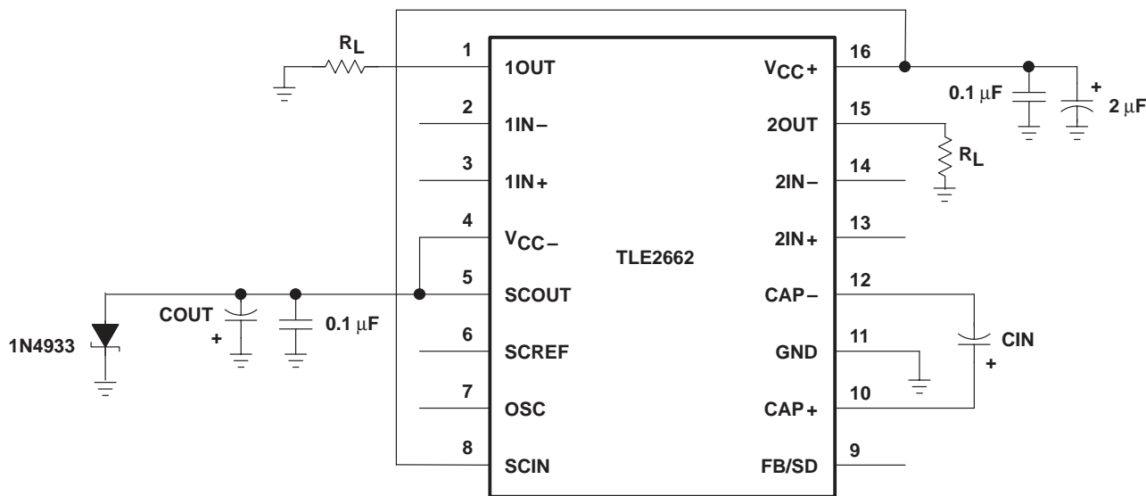
Figure 4. Test Circuit
