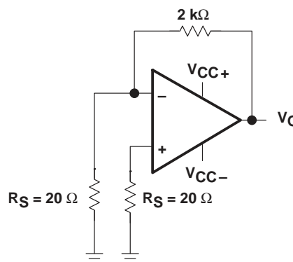
Figure 2. Noise-Voltage Test Circuit
