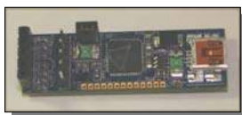
I2C-USB Bridge
