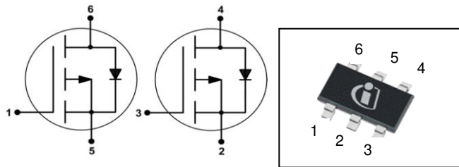
PG-TSOP6
