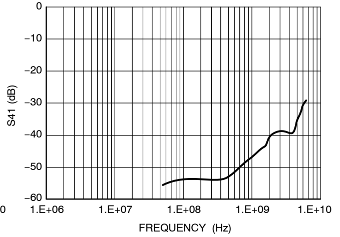
Figure 5. Analog Crosstalk Curve (S41 Measurement)
