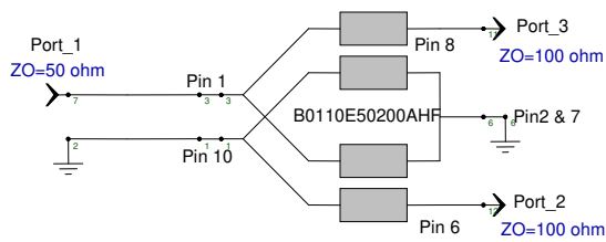
Figure 2 The Balun in it's basic configuration with no external components.
