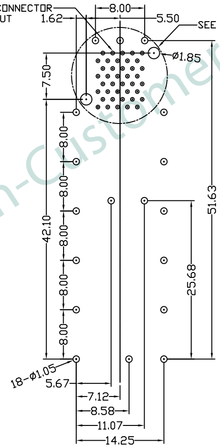
P.C.B LAYOUT TOP VIEW ±0.05
