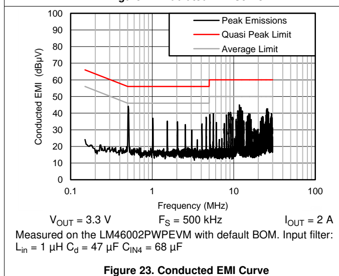
Figure 23. Conducted EMI Curve
