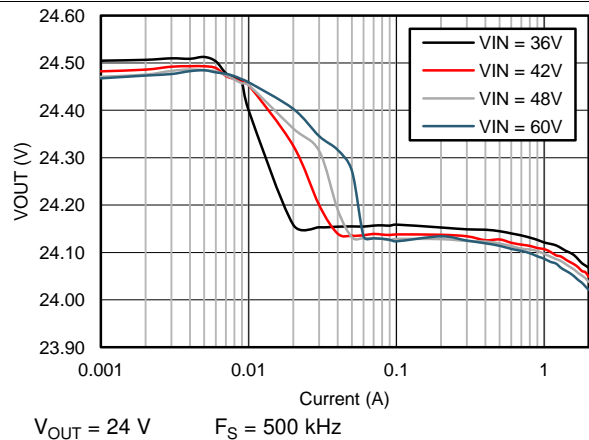
Figure 12. V_{OUT} Regulation
