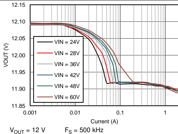
Figure 11. V_{OUT} Regulation
