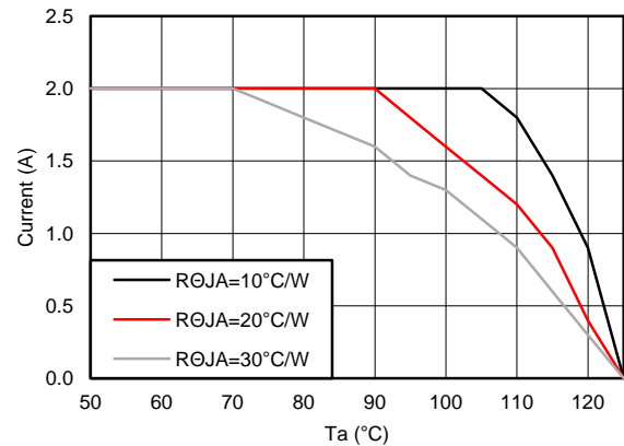
Figure 64. Derating Curve
