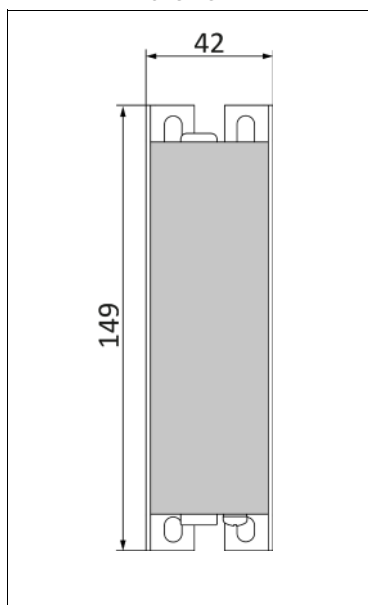
Fig. 24-4 Wall/panel mounting, front view
