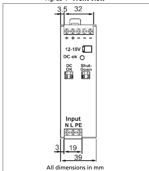
Fig. 23-1 Front view
