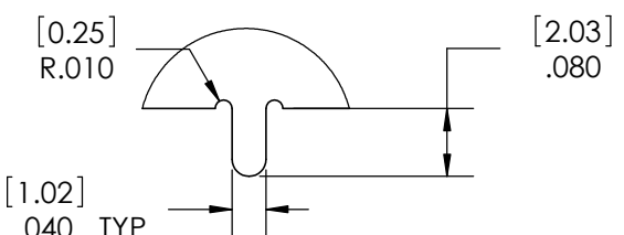
DETAIL A SCALE 4 : 1
