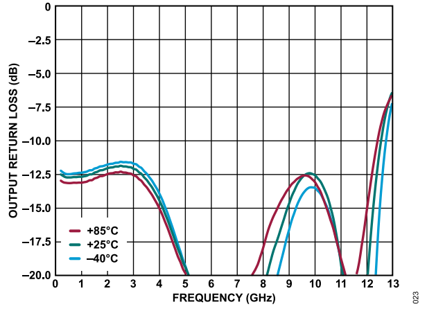
Figure 23. Output Return Loss vs. Frequency for Various Temperatures, 200 MHz to 13 GHz, V_{DD} = 5\text{ V} , I_{DQ} = 95\text{ mA}
