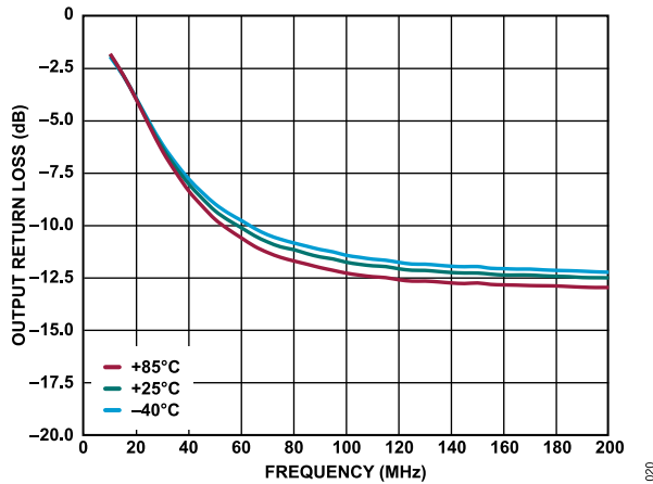
Figure 20. Output Return Loss vs. Frequency for Various Temperatures, 10 MHz to 200 MHz, V_{DD} = 5\text{ V} , I_{DQ} = 95\text{ mA}
