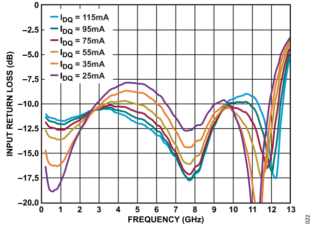
Figure 22. Input Return Loss vs. Frequency for Various I_{DQ} Values, 200 MHz to 13 GHz, V_{DD} = 5\text{ V}
