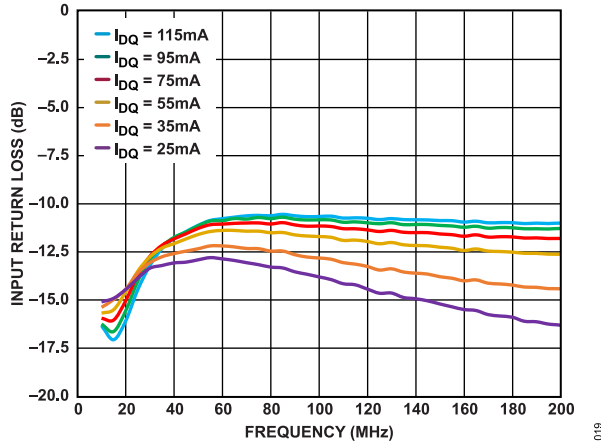
Figure 19. Input Return Loss vs. Frequency for Various I_{DQ} Values, 10 MHz to 200 MHz, V_{DD} = 5\text{ V}
