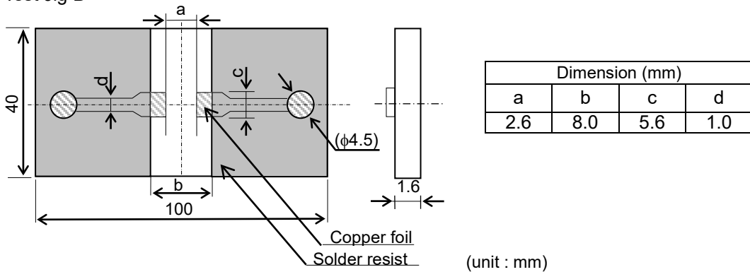
(2) Test Jig B
