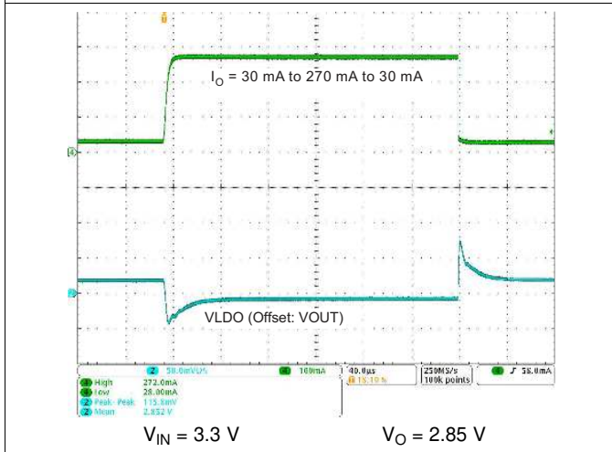
Figure 8-22. Load Transient Response LDO9
