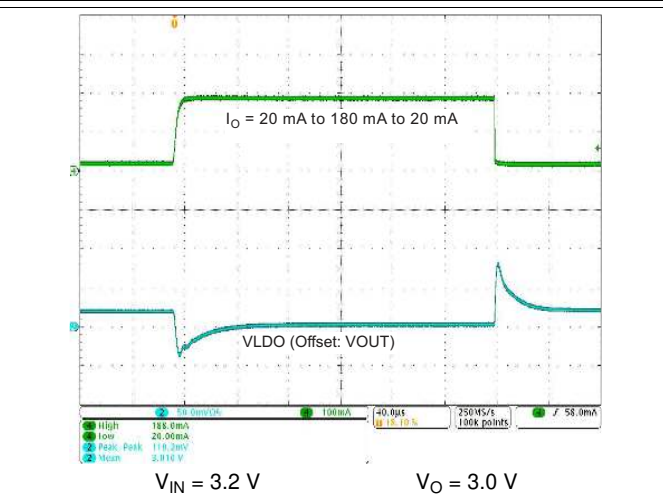
Figure 8-21. Load Transient Response LDO7
