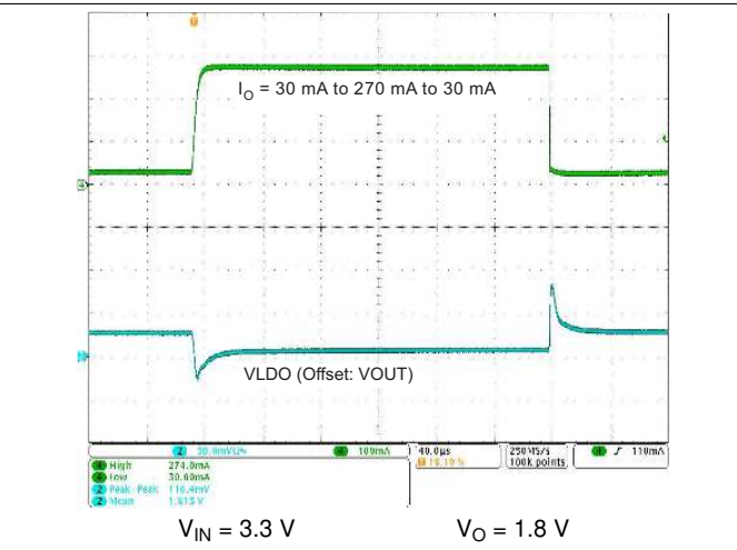
Figure 8-23. Load Transient Response LDO10
