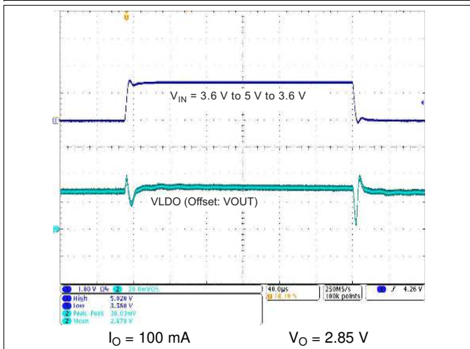
Figure 8-20. Line Transient Response LDO6, LDO8
