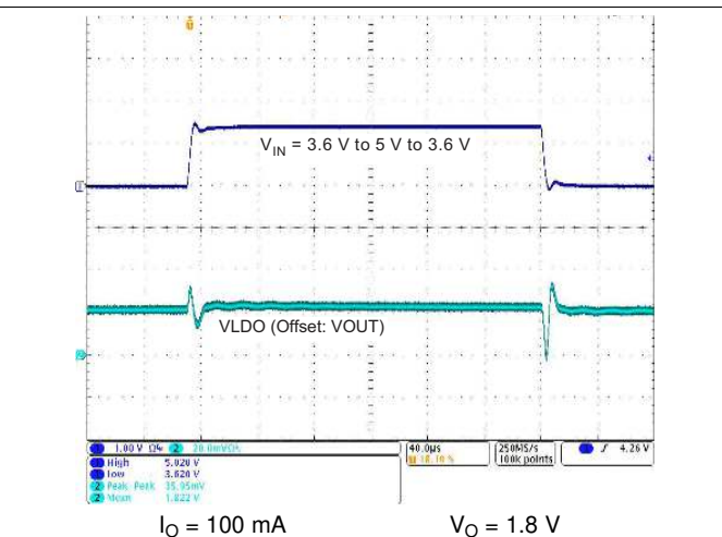
Figure 8-19. Line Transient Response LDO6, LDO8
