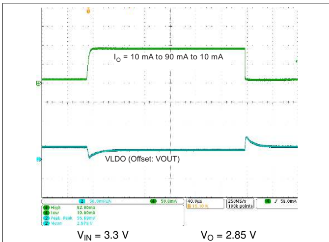
Figure 8-18. Load Transient Response LDO6, LDO8
