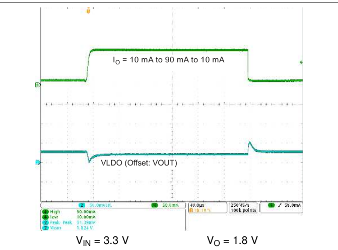
Figure 8-17. Load Transient Response LDO6, LDO8
