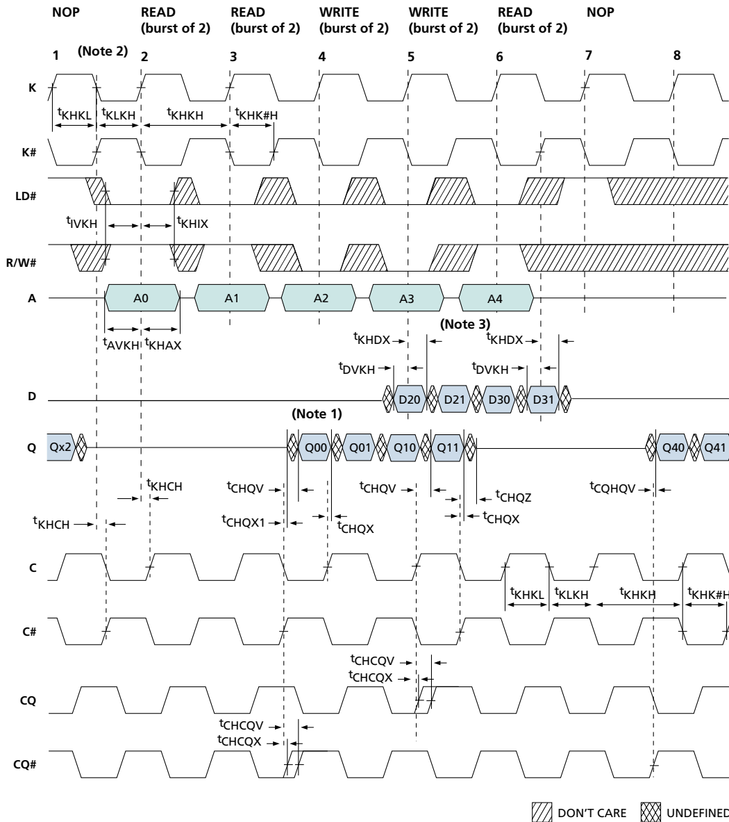
Figure 6: READ/WRITE Timing
