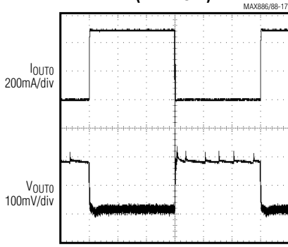
REG0 LOAD-TRANSIENT RESPONSE (PFM MODE)
