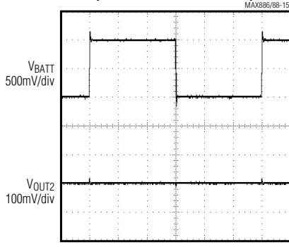
REG2 LINE-TRANSIENT RESPONSE (IN2 CONNECTED TO OUT0)
