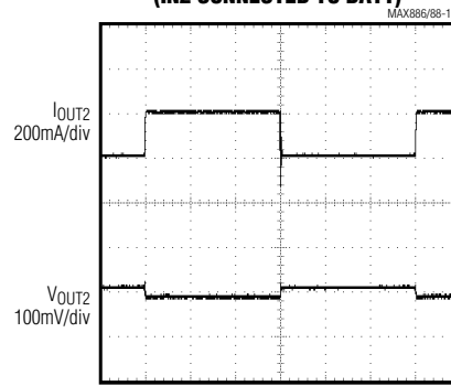
REG2 LOAD-TRANSIENT RESPONSE (IN2 CONNECTED TO BATT)
