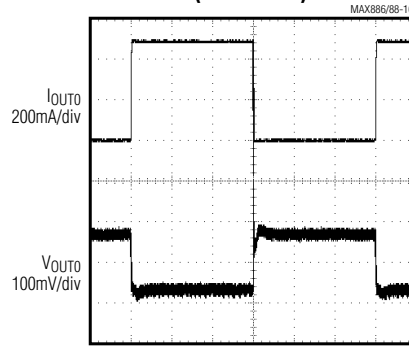
REG0 LOAD-TRANSIENT RESPONSE (PWM MODE)
