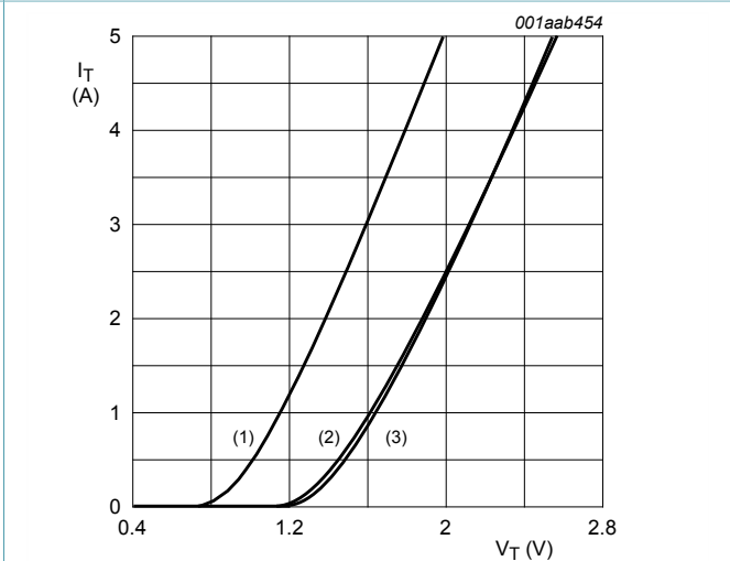
V_o = 1.067 \text{ V}; R_s = 0.187 \Omega (1) T_j = 125 \text{ }^\circ\text{C} ; typical values (2) T_j = 125 \text{ }^\circ\text{C} ; maximum values (3) T_j = 25 \text{ }^\circ\text{C} ; maximum values Fig. 10. On-state current as a function of on-state voltage
