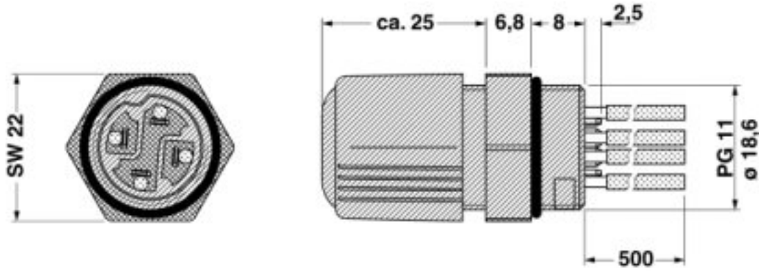
Dimensioned drawing
