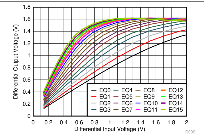
Figure 6-6. USB RX Linearity Curves at 2.5 GHz
