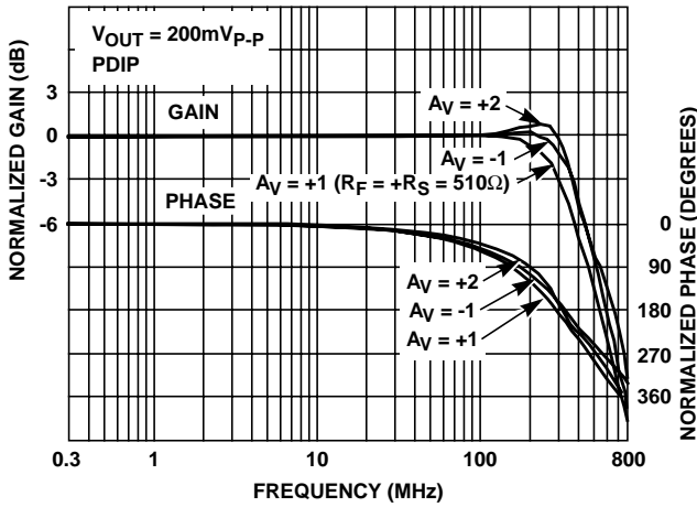
FIGURE 48. FREQUENCY RESPONSE
