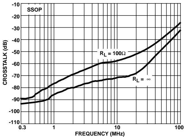
FIGURE 36. ALL HOSTILE CROSSTALK
