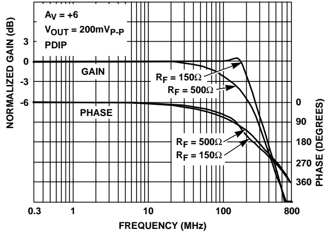
FIGURE 49. FREQUENCY RESPONSE
