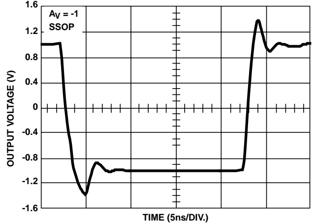
FIGURE 25. LARGE SIGNAL BIPOLAR PULSE RESPONSE
