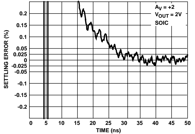
FIGURE 19. SETTLING RESPONSE
