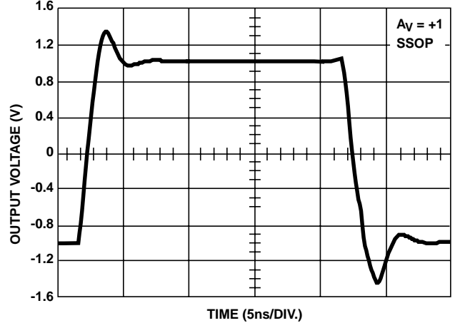
FIGURE 27. LARGE SIGNAL BIPOLAR PULSE RESPONSE
