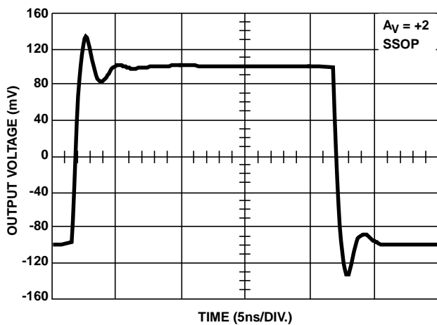
FIGURE 20. SMALL SIGNAL PULSE RESPONSE
