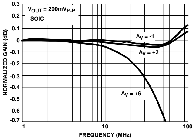
FIGURE 16. GAIN FLATNESS
