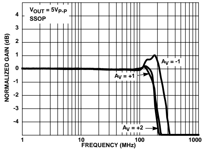
FIGURE 35. FULL POWER BANDWIDTH
