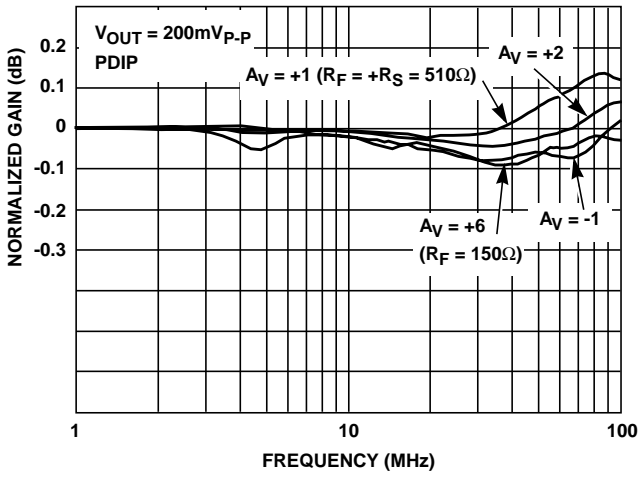
FIGURE 52. GAIN FLATNESS
