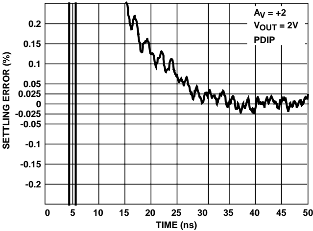
FIGURE 54. SETTLING RESPONSE
