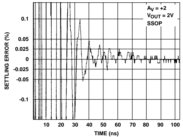
FIGURE 37. SETTLING RESPONSE
