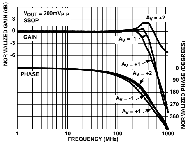
FIGURE 32. FREQUENCY RESPONSE
