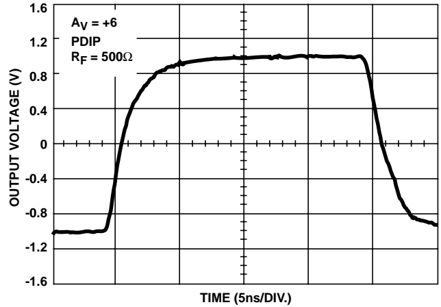
FIGURE 47. LARGE SIGNAL PULSE RESPONSE
