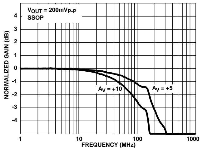
FIGURE 33. FREQUENCY RESPONSE
