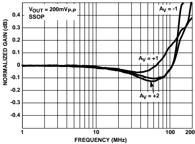
FIGURE 34. GAIN FLATNESS
