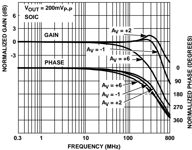
FIGURE 14. FREQUENCY RESPONSE
