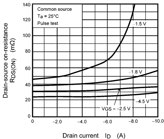
Fig. 7.5 R_{DS(ON)} - I_D
