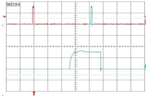
Figure 14. Load current (top trace, 20 A/div., 50 ms/div.) into a 10\ \text{m} short circuit during restart, at V_{in} = 48\ \text{V} . Bottom trace (20 A/div., 2 ms/div.) is an expansion of the on-time portion of the top trace
