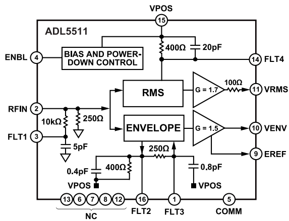
Figure 48. Block Diagram
