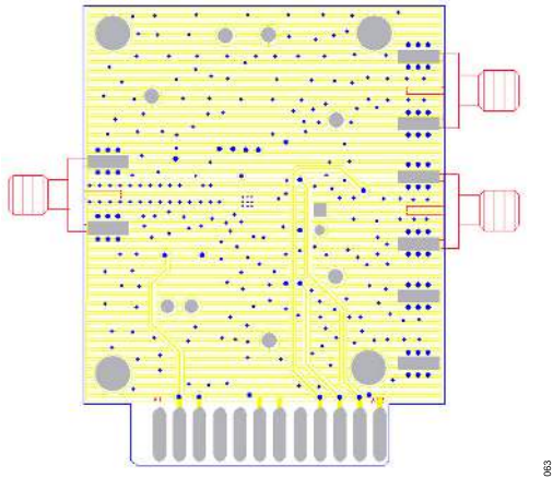
Figure 60. Layout of Evaluation Board, Bottom Side
