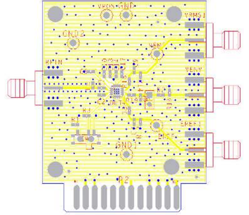
Figure 61. Layout of Evaluation Board, Top Side
