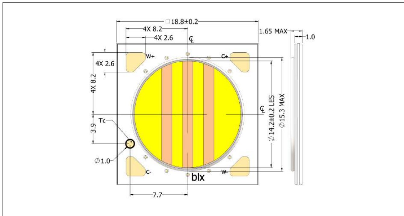
Figure 28: Drawing for Vesta Series Tunable White Gen 2 13mm Array
