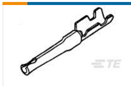
TE Part #1658686-1 SOCKET CONTACT,22 DF,STRIP,22-
