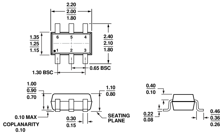
COMPLIANT TO JEDEC STANDARDS MO-203-AB Figure 66. 6-Lead Plastic Surface-Mount Package [SC70] (KS-6) Dimensions shown in millimeters
