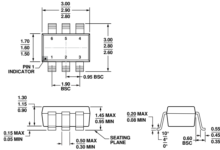
COMPLIANT TO JEDEC STANDARDS MO-178-AB Figure 65. 6-Lead Small Outline Transistor Package [SOT-23] (RJ-6) Dimensions shown in millimeters
