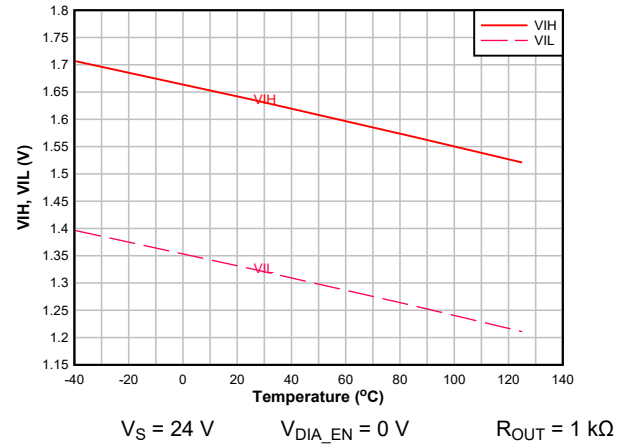
Figure 7-8. V_{IH} , V_{IL} vs Temperature
